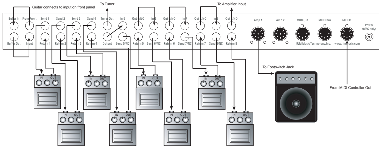
Setup 1 – Four FX Pedals, One Amplifier
