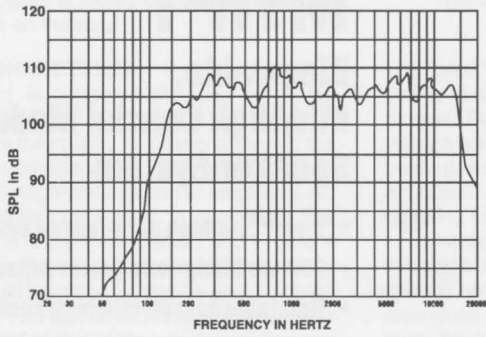
FIGURE 1 — Axial Frequency Response
