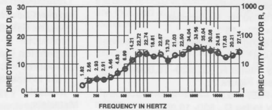
FIGURE 2 — Directivity vs Frequency (whole-space anechoic environment)
