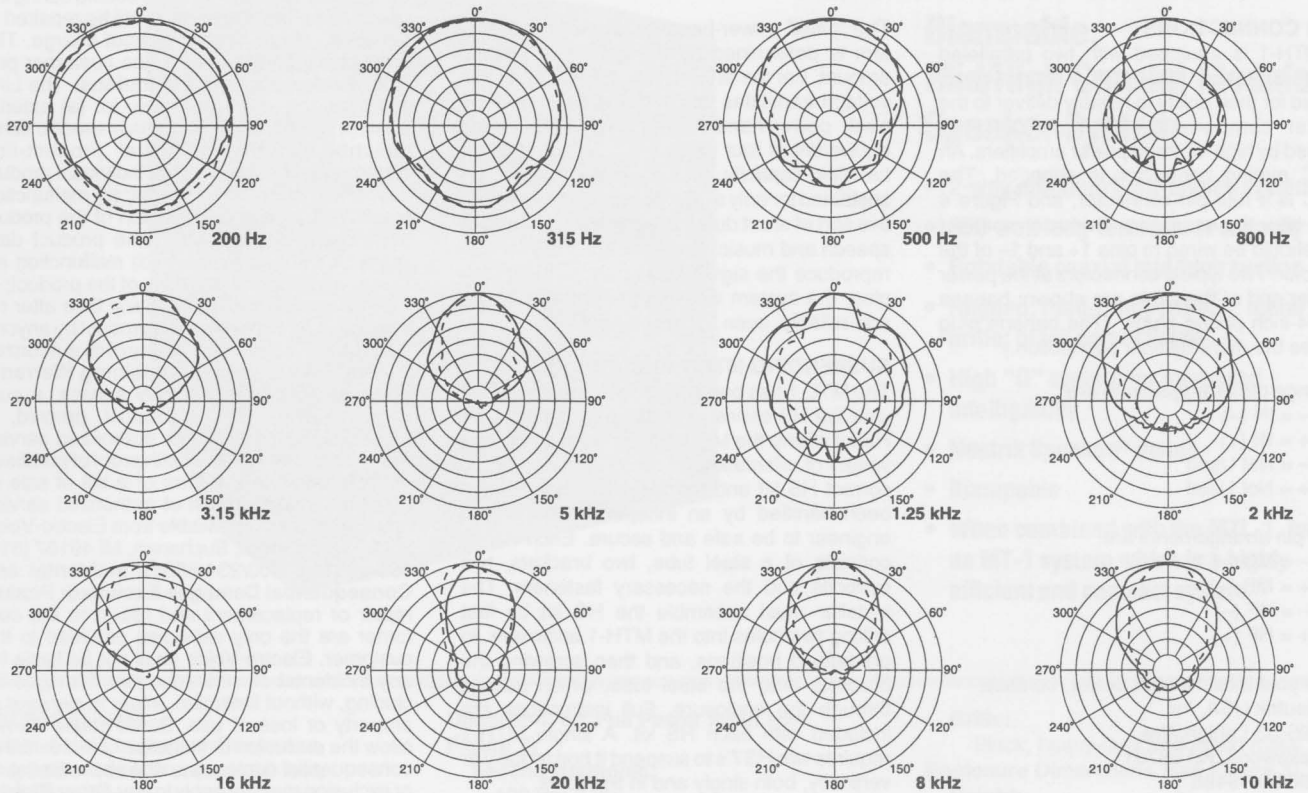
FIGURE 5 — One-Third-Octave Polar Responses (anechoic environment)
