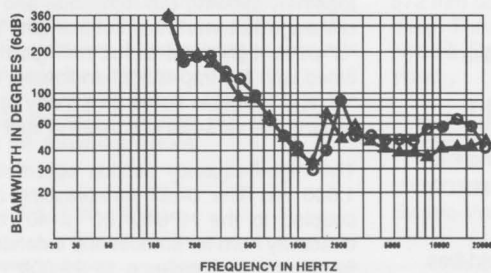
FIGURE 6 — Beamwidth vs Frequency (whole-space anechoic environment)
