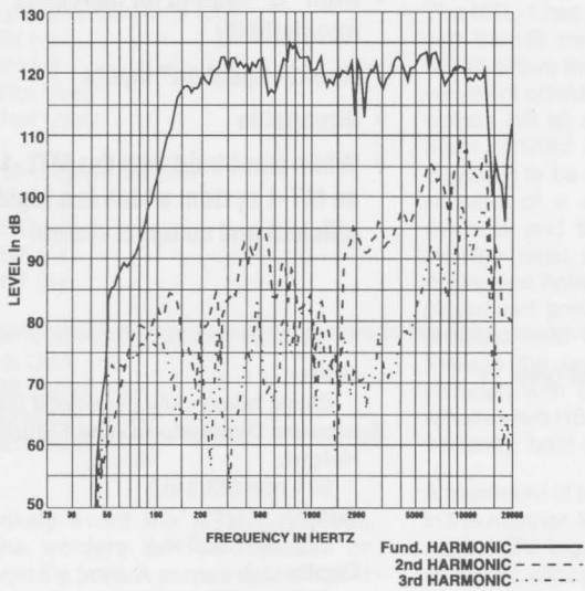
FIGURE 2 — Harmonic Distortion 0.1 Full Power Input
