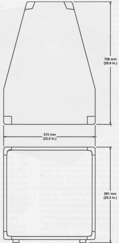
FIGURE 3 — Dimensions
